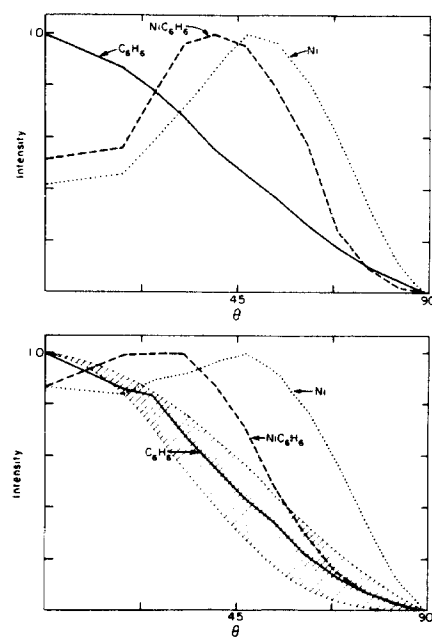
Figure 8. Polar angle distributions. The azimuthal angle of collection is along the (100) direction. The polar resolution is \pm 12.5^\circ . The top panel is from the SIMS simulation and the bottom from the PDMS simulation. The shaded area is bracketed by lines of \cos^{1.5} \theta and \cos^{3.5} \theta . Only particles with less than 20 eV of kinetic energy are collected.
