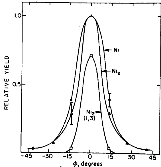
FIG. 4. Calculated angular distributions of \text{Ni} and \text{Ni}_2 at a polar angle of 45^\circ \pm 5^\circ . The center-of-mass kinetic energy is between 10 and 50 eV. Also shown is the contribution to the \text{Ni}_2 distributions from dimers formed on atoms No. 1 and No. 3 of Fig. 3. The peak intensity is 110 and 12 particles for the \text{Ni} and \text{Ni}_2 distributions, respectively.
