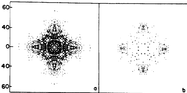
FIG. 3. Calculated angular distributions of \text{Ni}_2 . The ejected particles are displayed on a flat-plate collector an arbitrary distance above the surface. The radial distance is the polar ejection angle in degrees as given by the scale on the left. The orientation of the crystal is the same as in Fig. 4(a). (a) \text{Ni}_2 dimers of all T_{c.m.} are shown. (b) Only dimers of energy 10 \text{ eV} \leq T_{c.m.} \leq 50 \text{ eV} , are shown.
