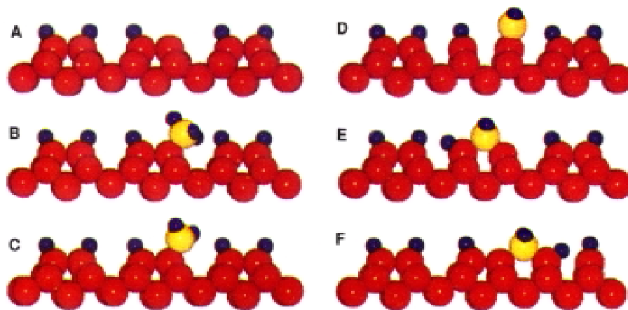
Fig. 1. Side view of the \{001\}(2\times 1) surface. In all cases the C atoms are represented by the larger spheres and the H atoms by the smaller spheres. The view angle is slightly off head-on. (A) Three surface dimers with an H atom on each dangling bond. (B) Surface dimer with a \text{CH}_3 replacing an H atom on the dangling bond. (C) Surface dimer with a \text{CH}_2 replacing an H atom on the dangling bond. (D) Same as (C) except that the surface dimer is open. (E) Insertion of the \text{CH}_2 into the dimer bond. (F) Insertion of the \text{CH}_2 into the trough position.
