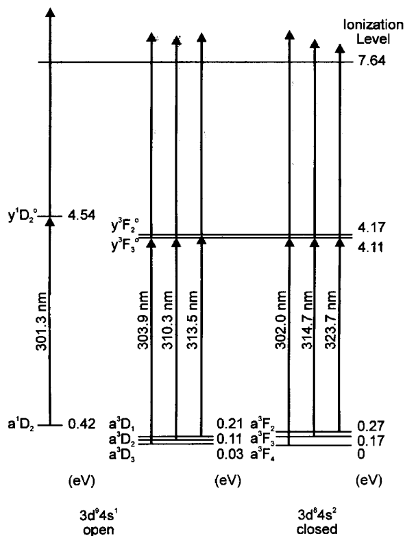
Figure 1. Partial electronic structure of atomic Ni showing the ionization schemes used in Ref. 27. The energy of each state above the ground state is noted in units of electron volts. 12
